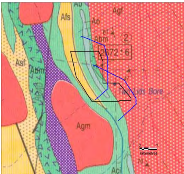
Figure 1. Layout of SAM survey with 1:250,000 scale GSWA solid geology map). The grid locations (black) and wire layout (blue) are indicated.
