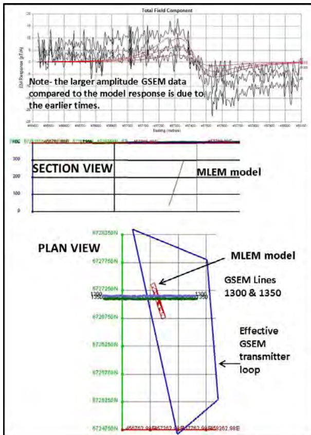
Figure 4. Northern 1000 target: Top panel – Channel 7-9 (15-80ms) GSEM response profiles (black) with MLEM model response profiles (red). Middle & bottom panels – Section & plan views of the MLEM plate model.
