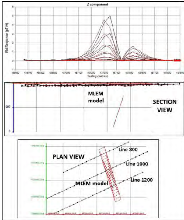
Figure 3. Northern 1000 target: Top panel – Channel 30-36 (45-220ms) in-loop MLEM response profiles (black) with MLEM model response (red). Middle & bottom panels – Section & plan views of the MLEM plate model.
