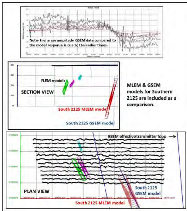
Figure 6. Western target: Top panel – Channel 7-9 (15-80ms) GSEM response profiles (black) with FLEM model response profiles (red). Middle and bottom panels – Section and plan views of the FLEM plate models.
