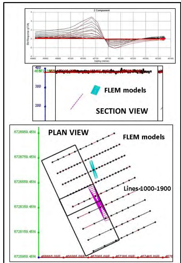
Figure 5. Western target: Top panel – Channel 25-36 (16-220ms) FLEM response profiles (black) with FLEM model response (red). Middle panel – Section view of FLEM plate models. Bottom panel – Plan view of FLEM models.
